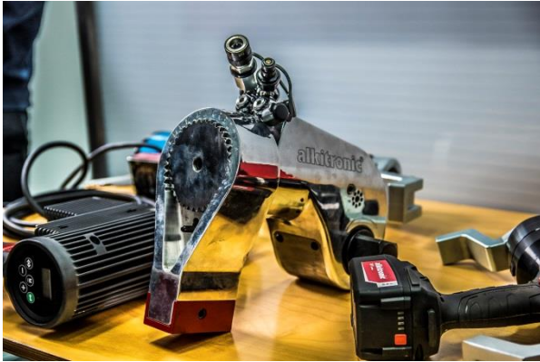
Figure 2: Presentation of alkitronic® torque multipliers
