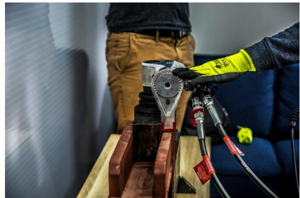
Figure 1: alkitronic® AS 3 Hydraulic torque multiplier in use during training
