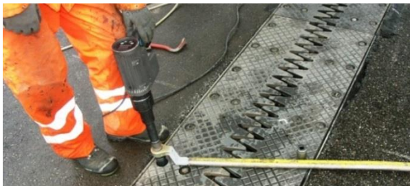
Figure 1: The ECip 100N at bridge construction
